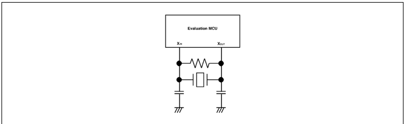
Figure 2.20 Circuit in which oscillation does not occur
